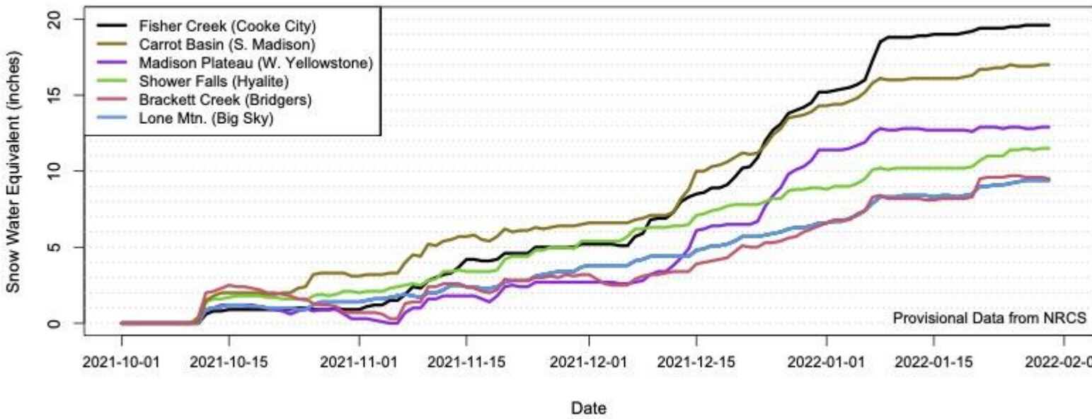
Graph of Snow Water Equivalent (SWE) at SNOTEL sites in the GNFA forecast area from October 1, 2021 to January 30, 2022. It highlights the extended dry conditions in January that contributed to weak layers forming at the top of the snowpack. GNFA
